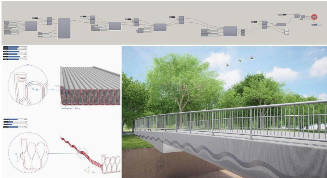
Figuur 3. Singapore 3DCP load bearing bridge (bron: Witteveen+Bos)
